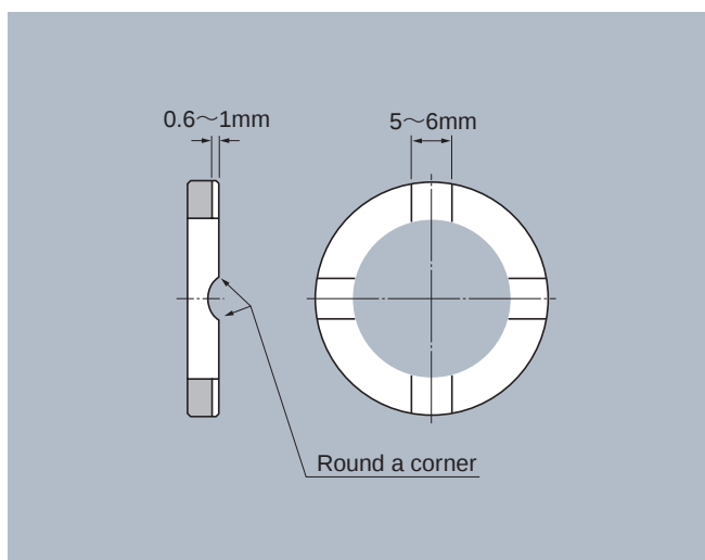
Fig. 7.3 Design of thrust ring guide surface
