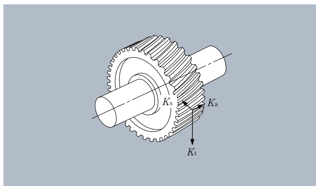
Fig. 3.2 Load acting on helical gear
