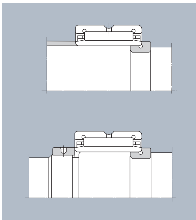
Fig. 7.8 Inner ring fixing by side ring
