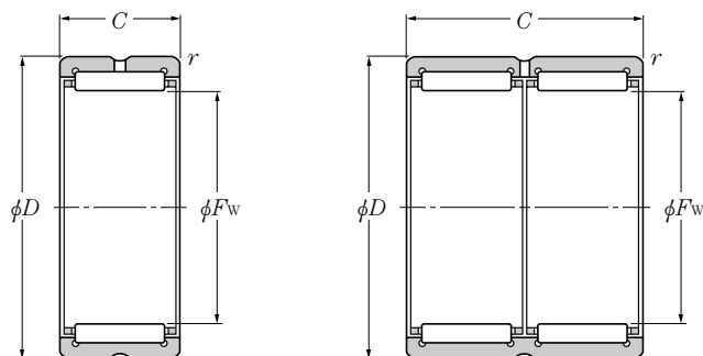
Type RNA48 Type RNA49·R, Type RNA69 RNA59 type Type NK·R, Type NK
