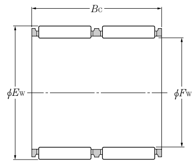
Type K··ZW
