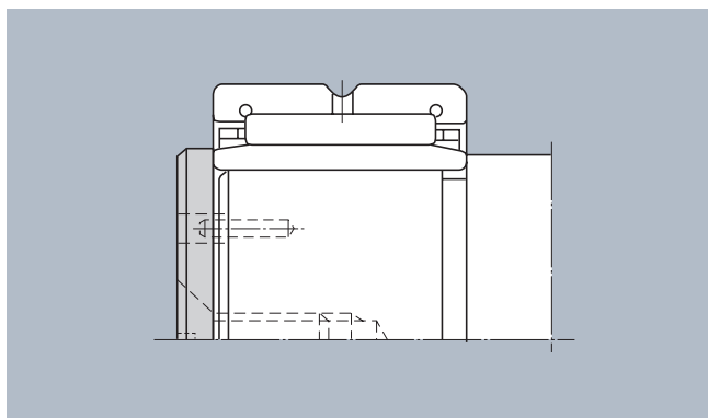
Fig. 7.7 Inner ring fixing by end plate
