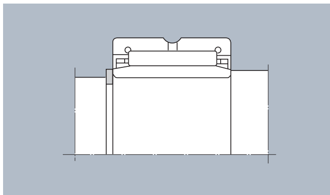
Fig. 7.6 Inner ring fixing by snap ring
