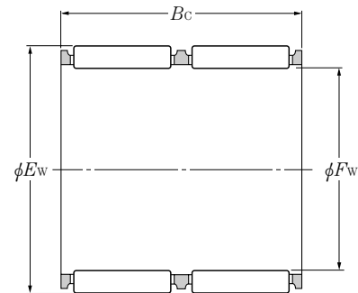
Type K··ZW
