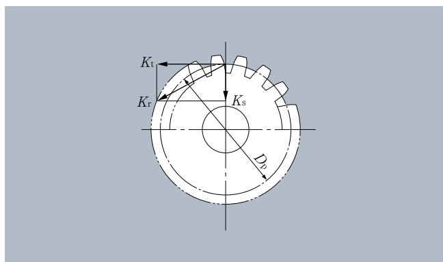
Fig. 3.3 Composite radial force acting on gear
