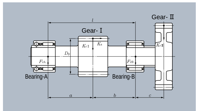
Fig. 3.7 Gear shaft
